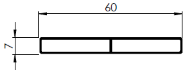
TRAV. BITULAR 60 x 7 x 1,2MM
