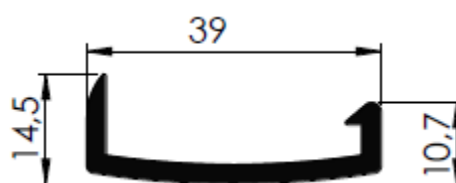
PERFIL LATERAL MESA 39 X 14,5MM
