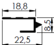
CASE 05 22,5 X 18,8MM
