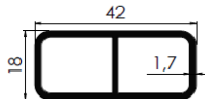
TRAV. BITUBULAR 42 X 18 X 1,7MM
