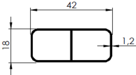
TRAV. BITUBULAR 42 X 18 X 1,2MM
