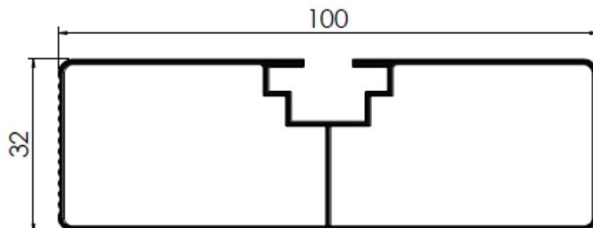
TRAVESSA LATERAL "COMERCIAL IV"
