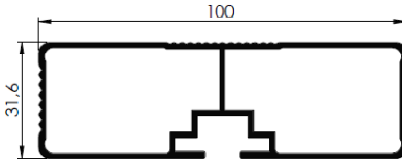
TRAVESSA LATERAL "COMERCIAL II"
