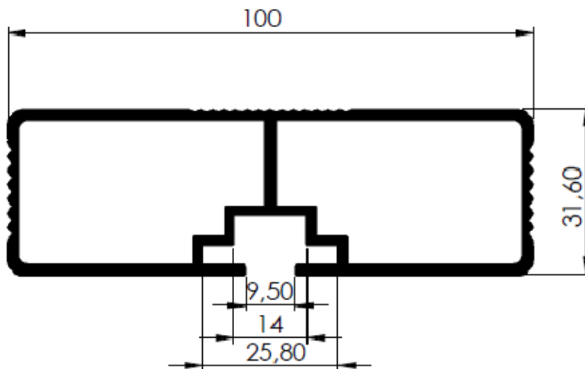
TRAVESSA LATERAL COMERCIAL
