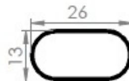
TUBO OBLONGO LISO 26,0 X 13 X 0,85
