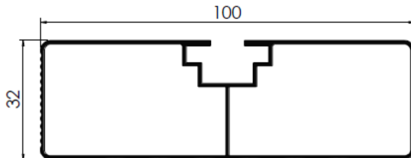
TRAVESSA LATERAL "COMERCIAL III"
