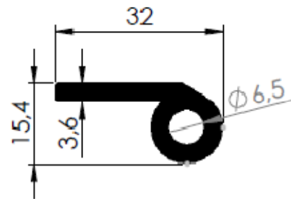
DOBRADIÇA 32 x 3,6MM
