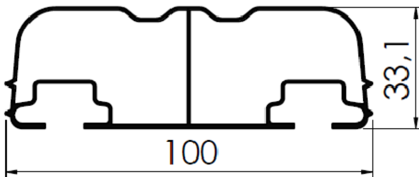
TRAVESSA LATERAL T-3687
