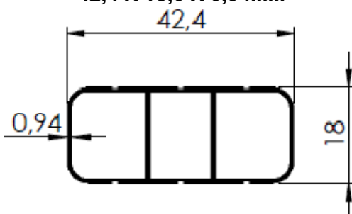
TRAV. TRITUBULAR C/ FRISO EXT. 42,4 X 18,0 X 0,94MM
